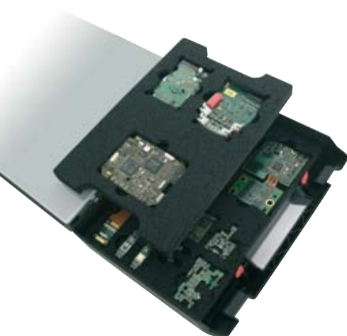
Antistatic foam in Plastazote LD 32 CN.
